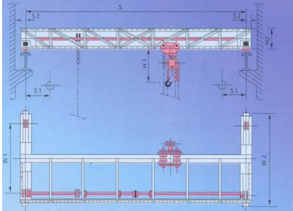
LEADING DIMENSIONS OF S.G. HOT CRANES
